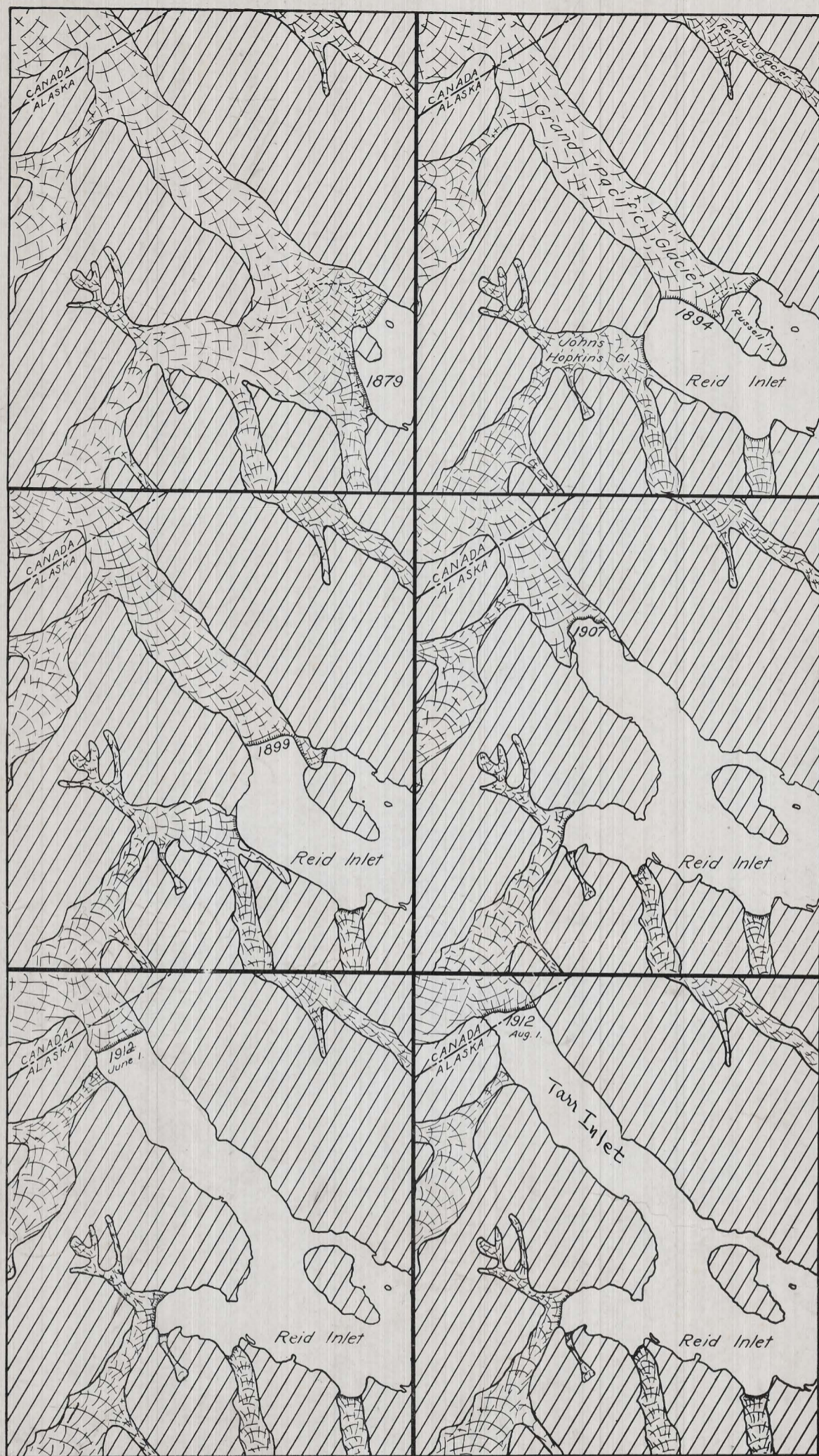
Grand Pacific Glacier, Tan Inlet, Glacier Bay, Alaska, 1879-1912, from Scientific American Supplement , Vol. 76, 1913, pp. 129, 136-138.
